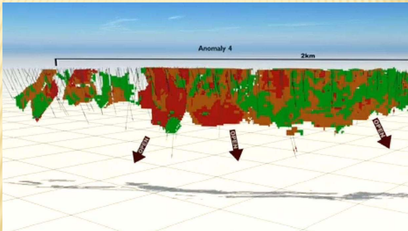
ANOMALY 4 MINERAL RESOURCES - VERTICAL SECTION (ALONG STRIKE)
